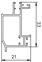
HANDLE PROFILE
