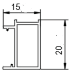
RECEIVER PROFILE
