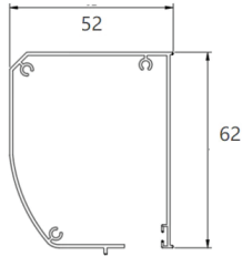
CASSETTE PROFILE
